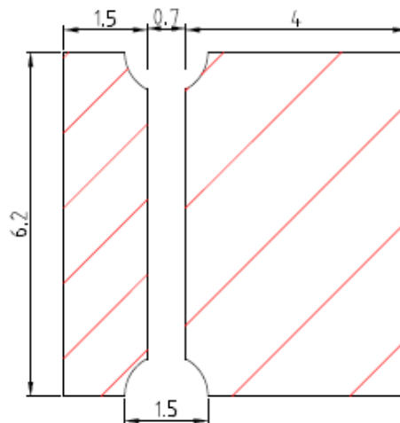
Recommended Stencil Pattern
