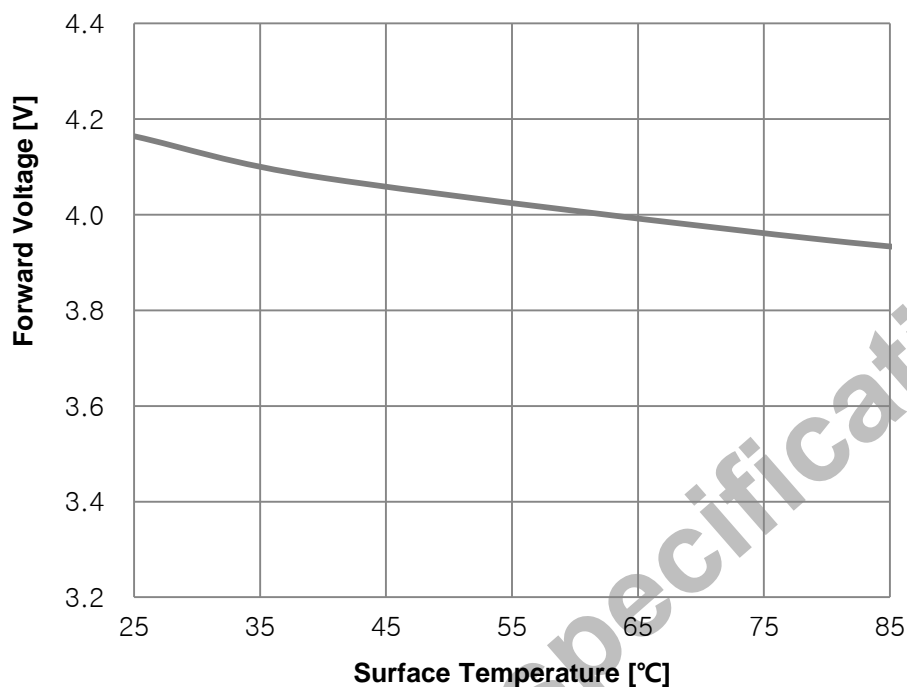
Fig 7. Surface Temperature vs. Forward Voltage, I_F=500\text{mA}
