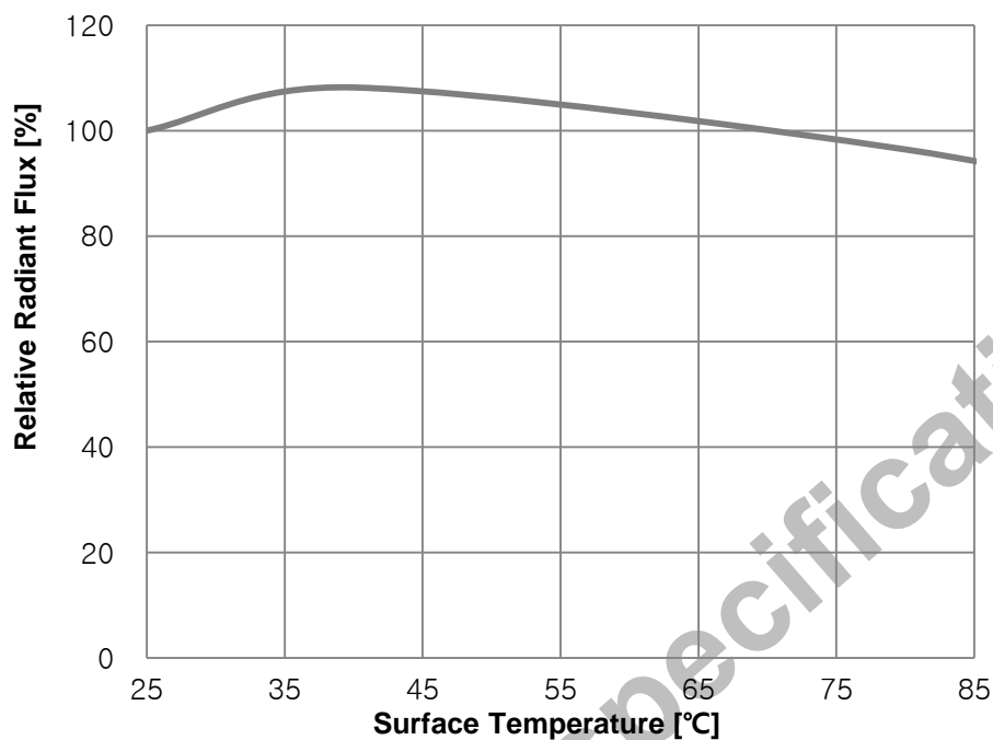
Fig 5. Surface Temperature vs. Relative Radiant Flux, I_F=500\text{mA}
