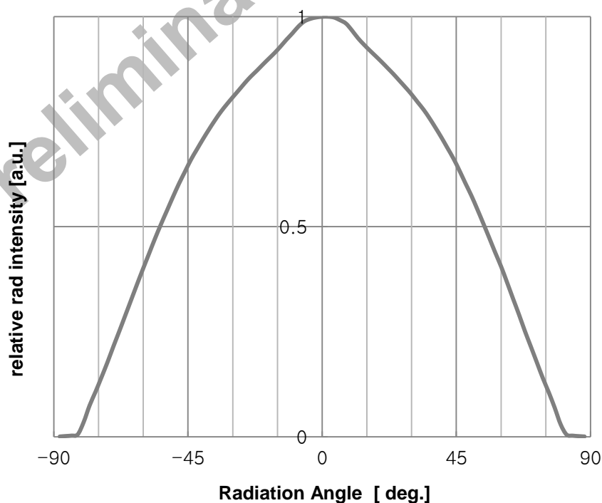
Fig 8. Typical Spatial Distribution, I_F=500\text{mA}
